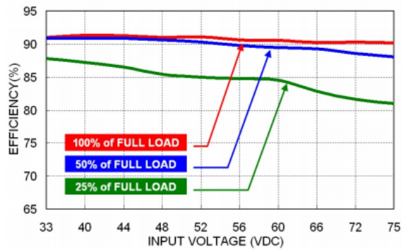
43 QAE100-48S05 Efficiency vs. Input Voltage
