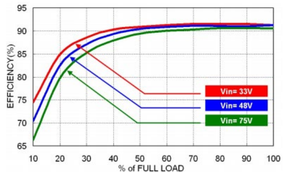
43 QAE100-48S05 Efficiency vs. Output Load
