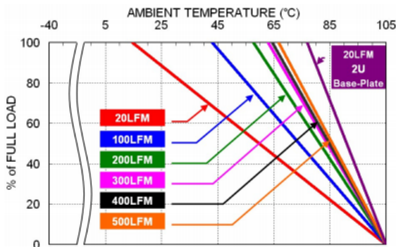
43 QAE100-48S05 Derating Curve
