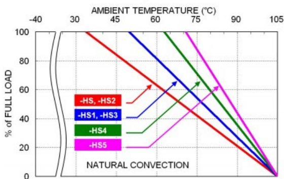
43 QAE100-48S05 Derating Curve with Heat-sink (See Thermal Considerations)
